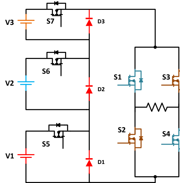
Fig. 1: The circuit diagram of the 15-level inverter.
